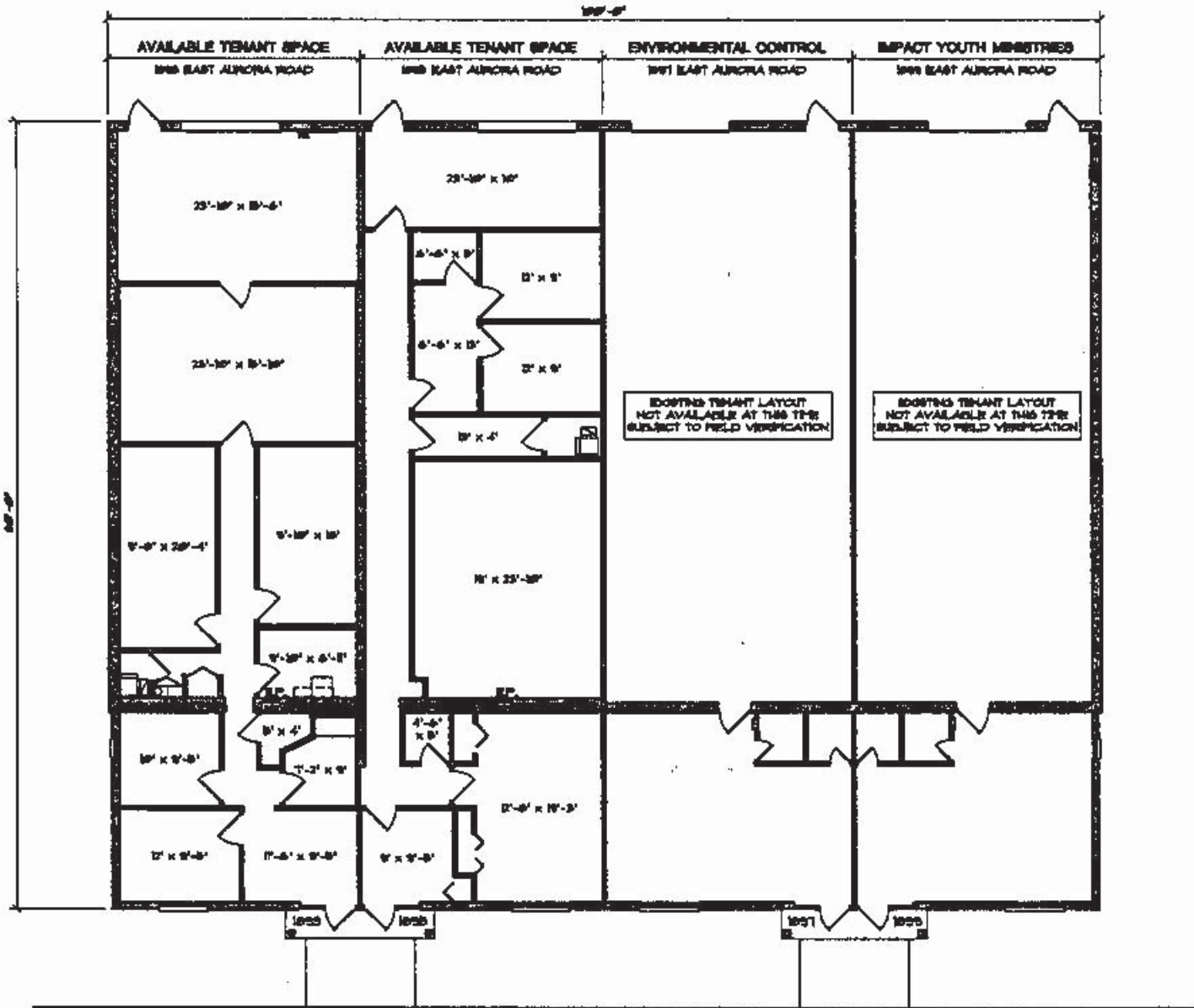
Building #1 Floor Plan
